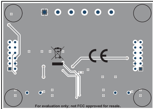
Figure 6-7. SENS063 Bottom View
