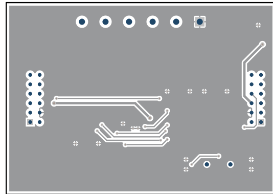
Figure 6-12. SENS064 Bottom Layer
