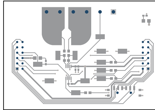
Figure 6-10. SENS064 Top Layer
