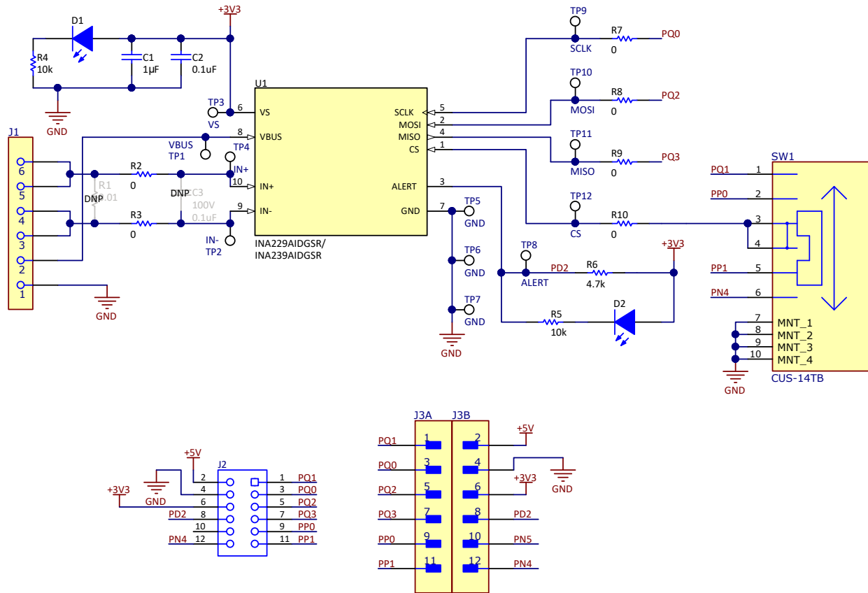
Figure 6-3. SENS064 Schematic
