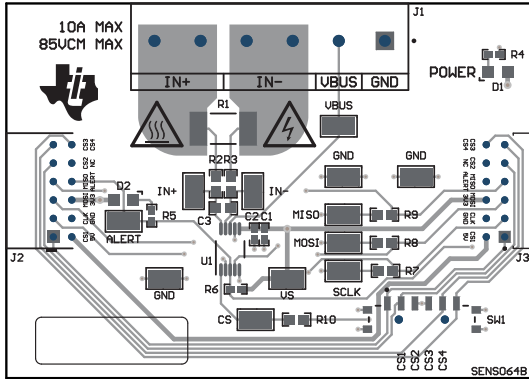
Figure 6-9. SENS064 Top View
