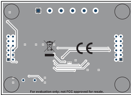
Figure 6-11. SENS064 Bottom View
