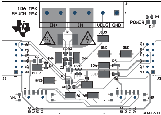
Figure 6-5. SENS063 Top View
