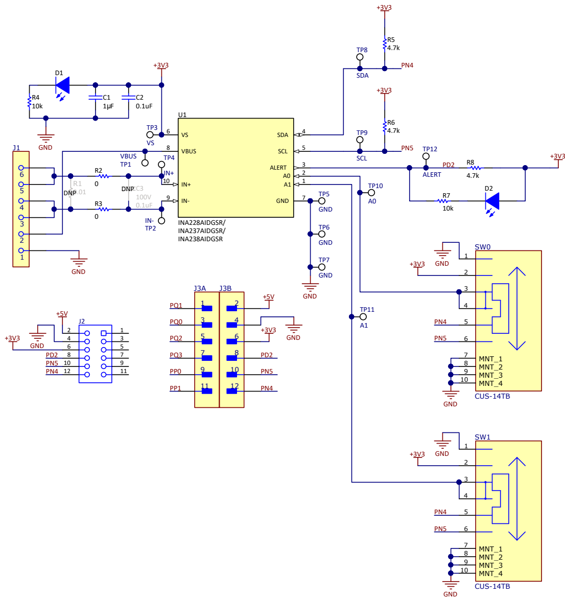
Figure 6-1. SENS063 Schematic
