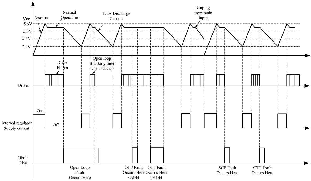
Figure 13: Signal Evolution Resulting from Faults
