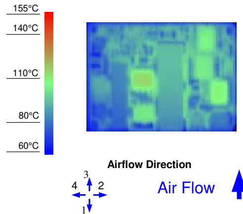
Figure 8. Thermal Image for Airflow Direction 3 (13.9A output, 55°C ambient, 0 LFM, typical Vin, open frame, unit soldered onto a fixture board)
