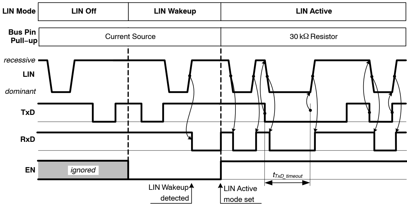
Figure 3. LIN Modes
