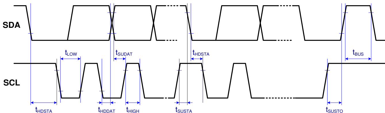
Figure 15. Bus Timing
