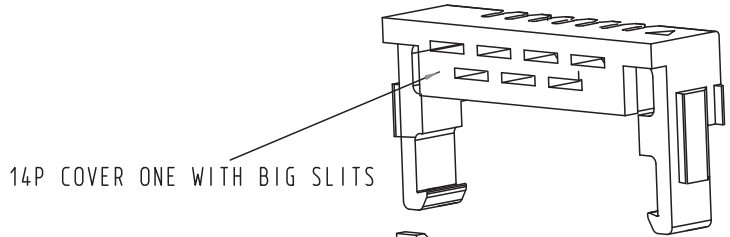
14P Har.Mik Bellow IDC Male Connector
