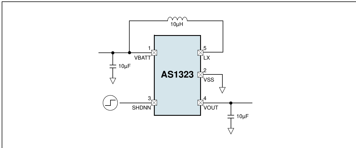
Figure 20. Typical Application
