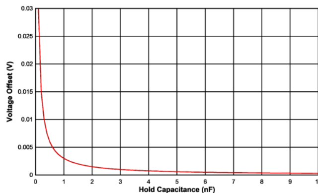
Figure 9-2. Sample-and-Hold Pedestal Error With 3-pC Charge Injection
