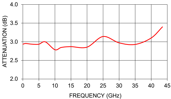
KAT-3+ ATTENUATION
