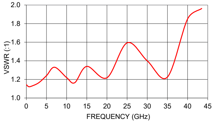
KAT-3+ VSWR
