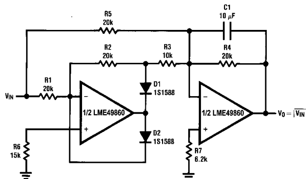
Figure 121. AC/DC Converter
