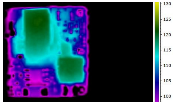
Figure 6. Thermal Image of CP30B1225036 2.5A output, 70C Ambient, 200lfm airflow, Vin = 48V, T_{max} = 122^{\circ}C
