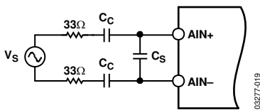
Figure 35. Simple ADC Drive Configuration
