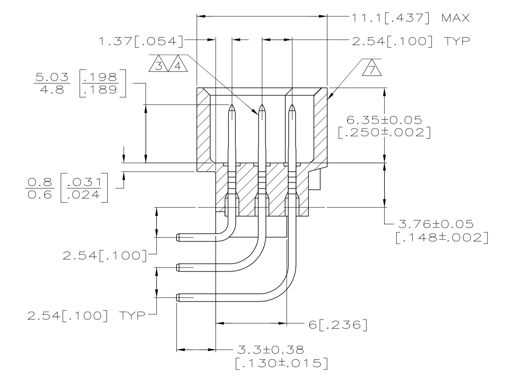
SECTION Z-Z
