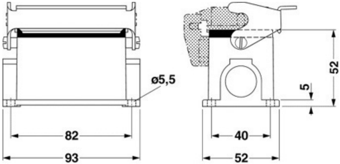
Dimensioned drawing
