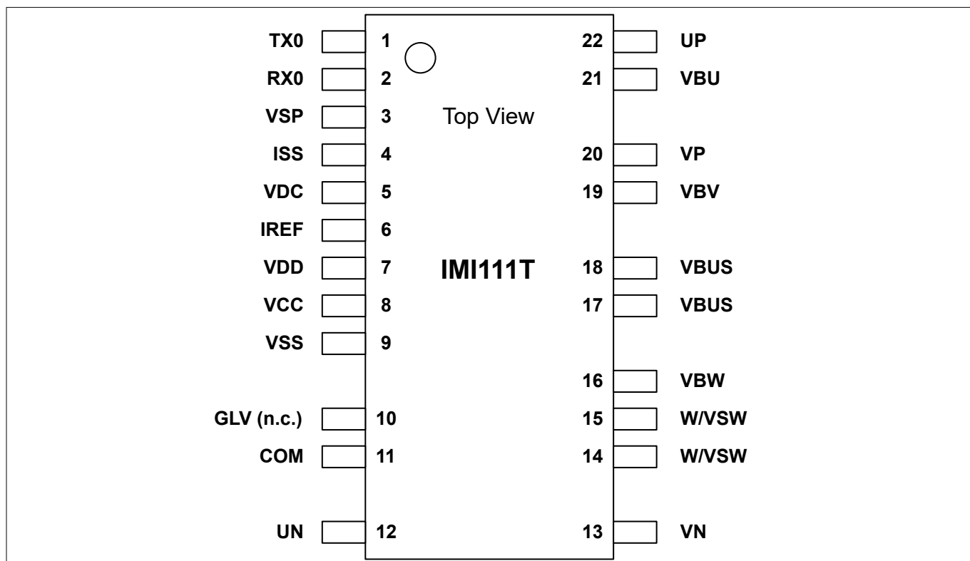
Figure 3 Pin assignment
