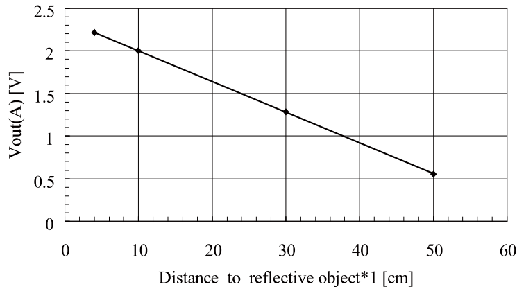
Example of output distance characteristics of GP2Y0E02A
