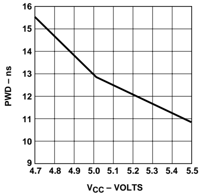
Figure 9. Typical POE receiver pulse width distortion vs. power supply voltage at high optical power, (0 dBm, 10 MBd).
