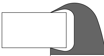
Too much solder Pad geometry too large
