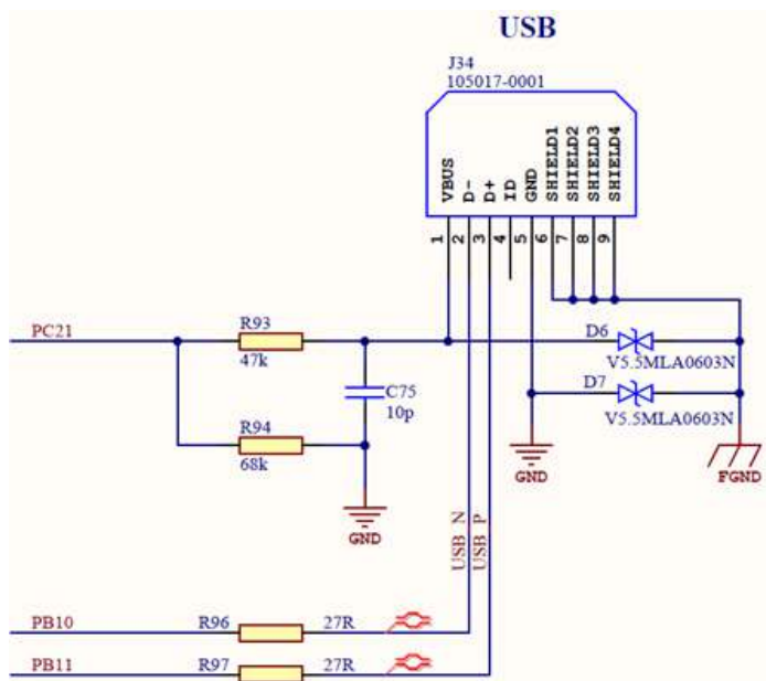
Figure 4-15. USB
