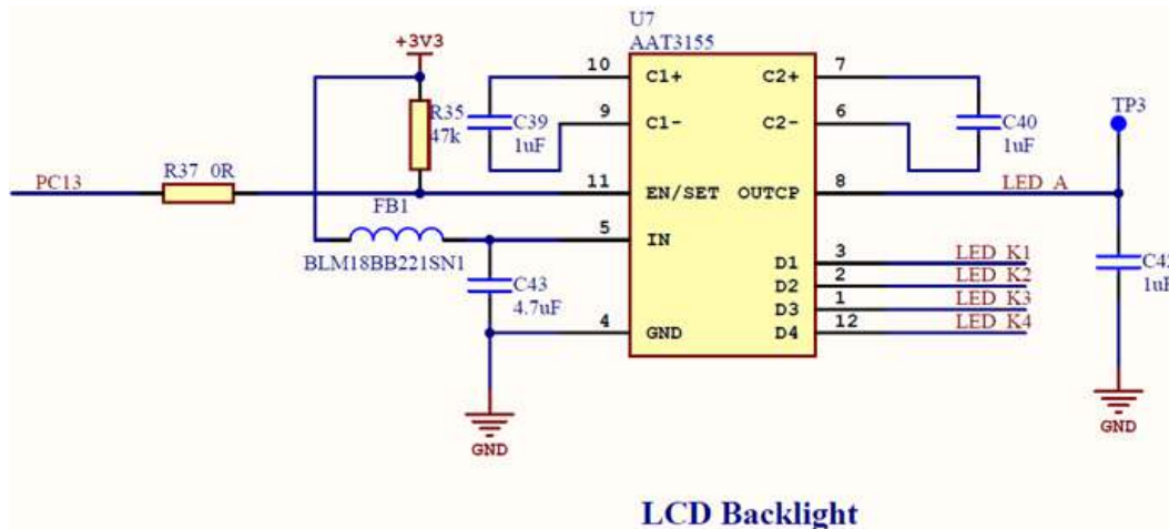
Figure 4-11. Backlight Control
