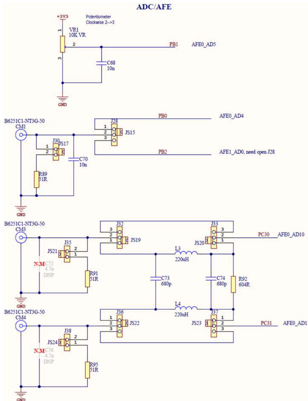
Figure 4-17. ADC/AFE Input
