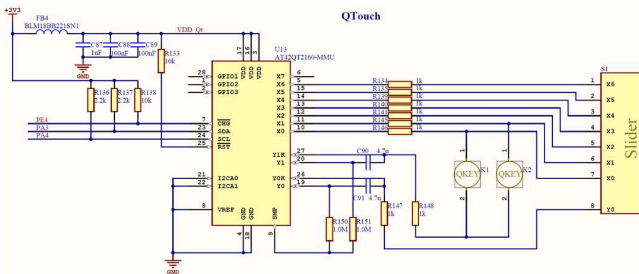
Figure 4-19. QT_Slider
