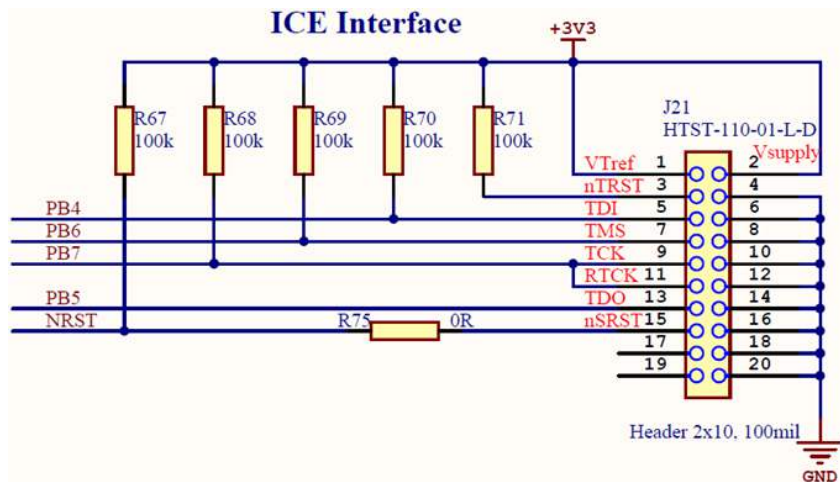
Figure 4-13. JTAG Interface
