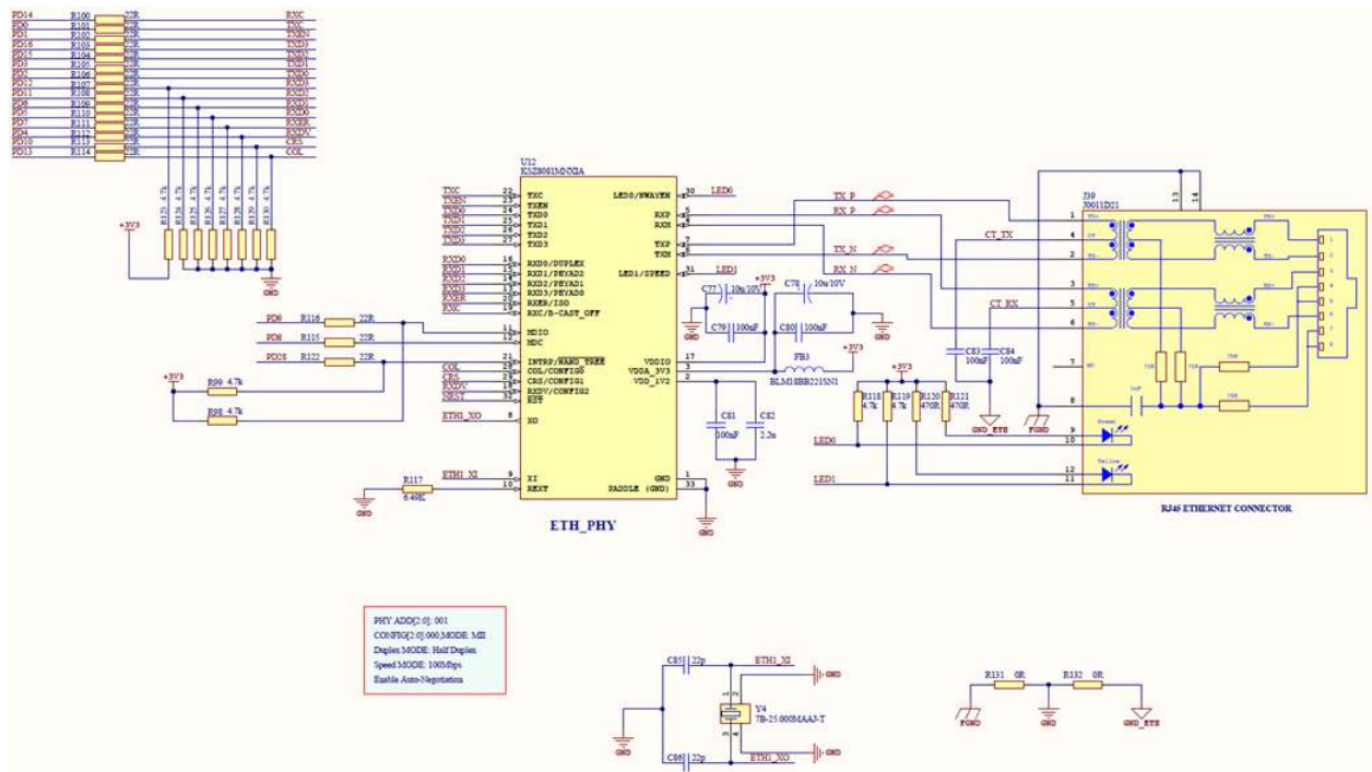
Figure 4-8. Ethernet Block
