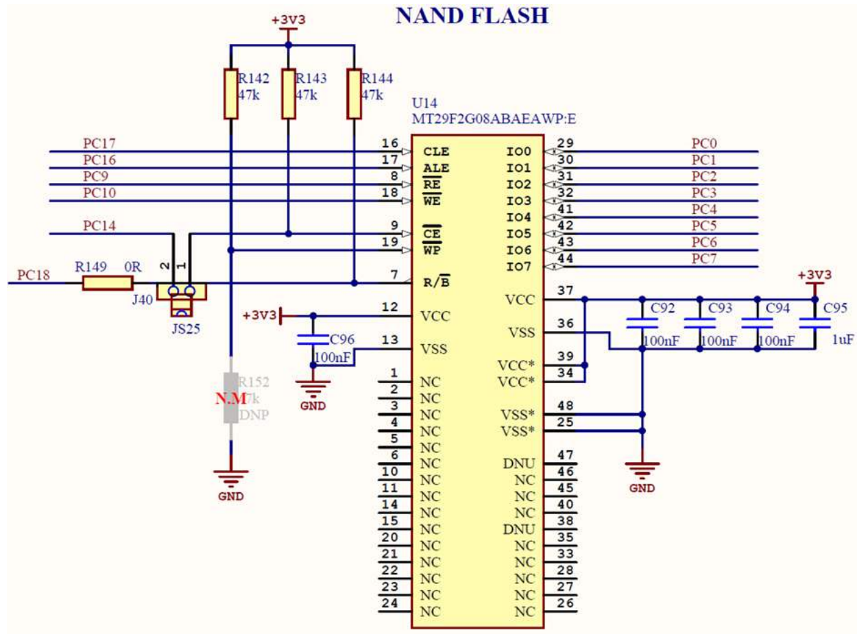
Figure 4-2. NAND-Flash
