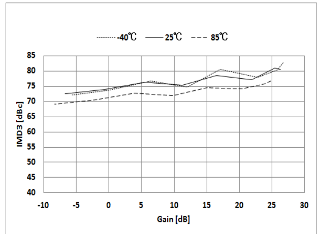
Figure.7-2 IMD3 VS Gain (fo=165MHz)
