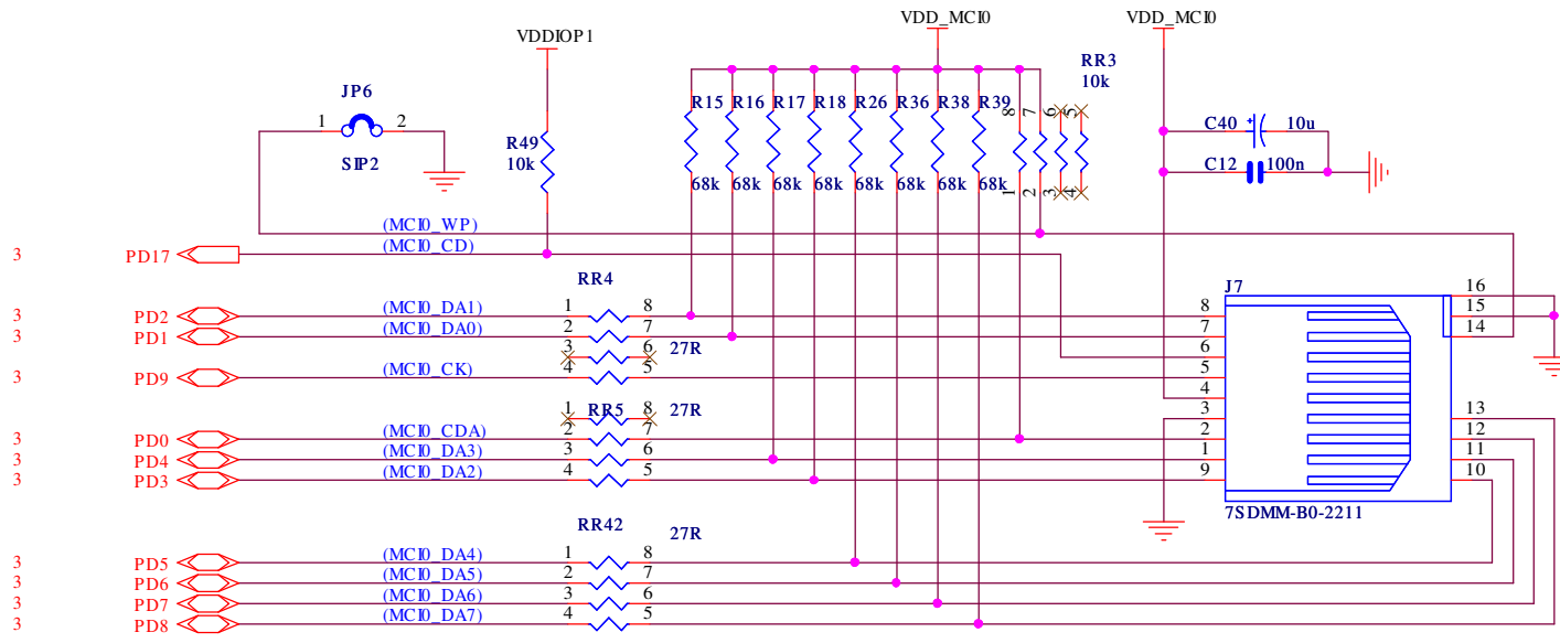
SD/MMCPlus CARD INTERFACE - MCIO
