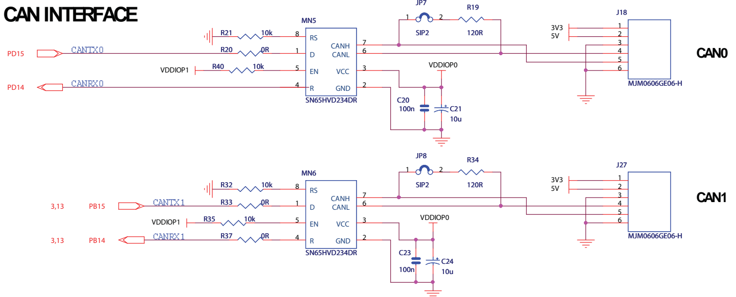
Figure 5-15. CAN on MB
