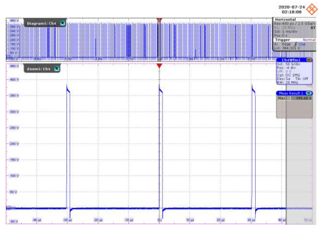
Figure 39 – Freewheeling Diode Voltage Waveforms. 265 VAC, 550 mA Output. 50 V / div., 10 µs / div. V_{MAX} : 395.7 V.
