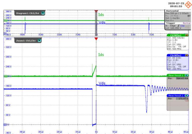
Figure 23 – Drain Voltage and Current Waveforms. 115 VAC, 0 mA Output. Upper: I DS , 400 mA / div. Lower: V DS , 40 V / div., 10 μs / div. I DS(MAX) = 0.564 A, V DS(MAX) = 171.1 V.
