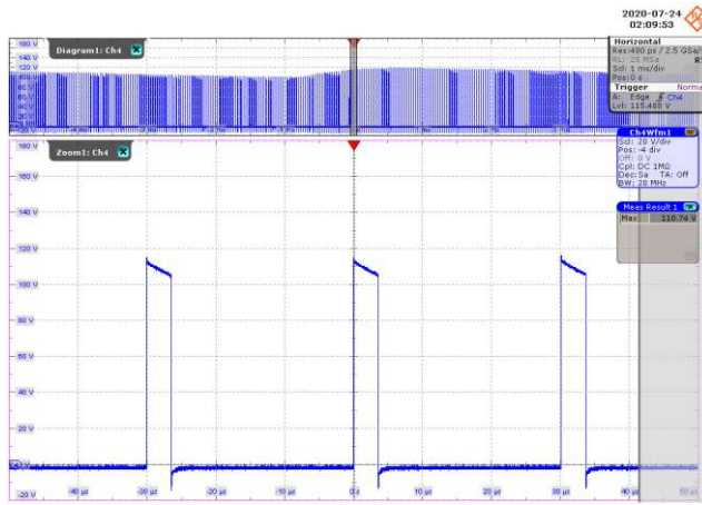
Figure 36 – Freewheeling Diode Voltage Waveforms. 85 VAC, 550 mA Output. 20 V / div., 10 µs / div. V_{MAX} : 118.7 V.
