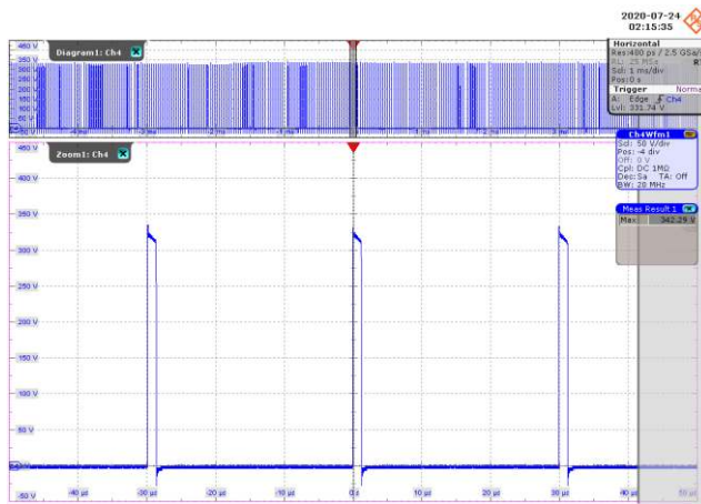
Figure 38 – Freewheeling Diode Voltage Waveforms. 230 VAC, 550 mA Output. 50 V / div., 10 µs / div. V_{MAX} : 342.3 V.
