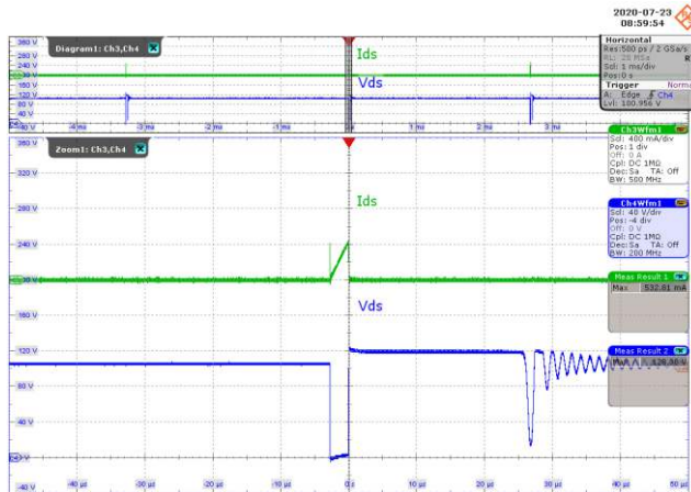
Figure 22 – Drain Voltage and Current Waveforms. 85 VAC, 0 mA Output. Upper: I DS , 400 mA / div. Lower: V DS , 40 V / div., 10 μs / div. I DS(MAX) = 0.532 A, V DS(MAX) = 128.4 V.
