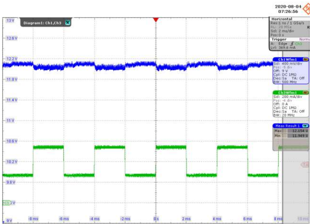
Figure 91 – Transient Output Waveforms. 230 VAC. Upper: V_{OUT} , 400 mV / div., 2 ms / div. Lower: I_{OUT} 200 mA / div. Load Transient: 50 % - 100%. Duty Cycle, Slew Rate: 50%, 0.8 A / \mu s. Frequency: 250 Hz. V_{MAX} : 12.15 V, V_{MIN} : 11.95 V.
