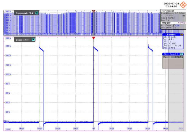
Figure 37 – Freewheeling Diode Voltage Waveforms. 115 VAC, 550 mA Output. 20 V / div., 10 µs / div. V_{MAX} : 171.7 V.
