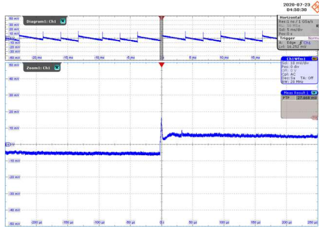
Figure 76 – Output Voltage Ripple Waveforms. 115 VAC, 0 mA Output. 10 mV, 5 ms / div.; 50 µs / div. V_{PK-PK} : 27.7 mV.
