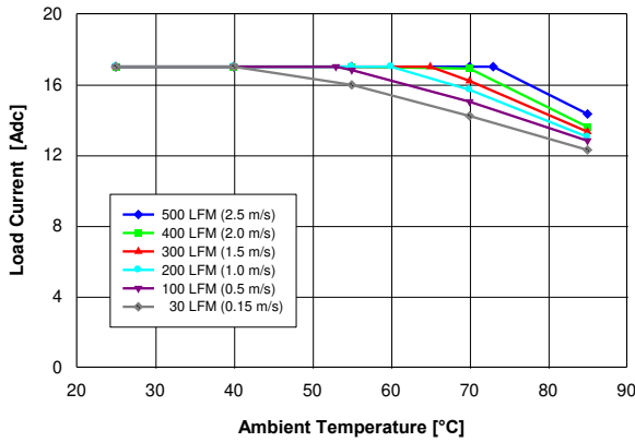
Fig. 1: Available load current vs. ambient air temperature and airflow rates for converter with G height pins mounted vertically with air flowing from pin 1 to pin 3 and maximum FET temperature \le 120\text{ }^\circ\text{C} , V_{in} = 48\text{ V} .
