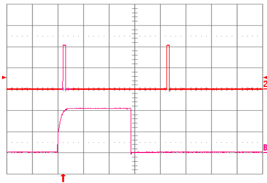
Fig. 16: Load current (top trace, 10 A/div., 50 ms/div.) into a 10 m\Omega short circuit during restart, at V_{in} = 48 V. Bottom trace (10 A/div., 2 ms/div.) is an expansion of the on-time portion of the top trace.
