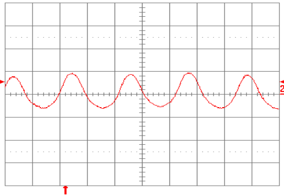
Fig. 13: Input reflected ripple current, i_c (100 mA/div.), measured at input terminals at full rated load current and V_{in} = 48 V. Refer to Fig. 12 for test setup. Time scale: 1 \mu s/div.
