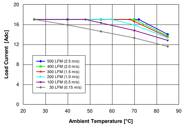
Fig. 2: Available load current vs. ambient air temperature and airflow rates for converter with G height pins mounted horizontally with air flowing from pin 1 to pin 3 and maximum FET temperature \le 120\text{ }^\circ\text{C} , V_{in} = 48\text{ V} .
