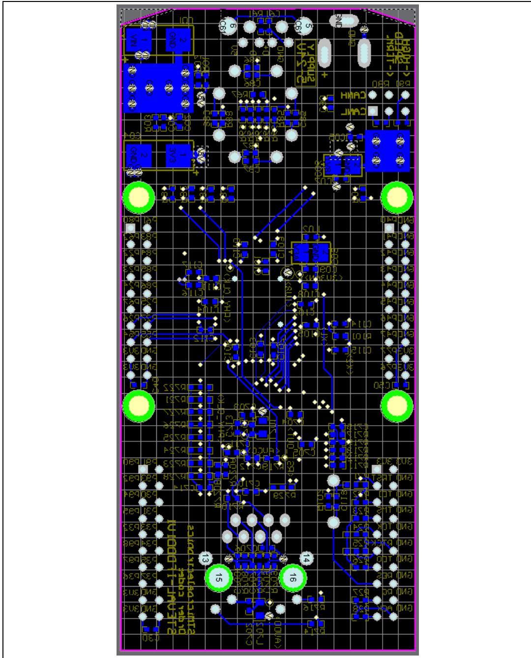
Figure 8. Bottom view
