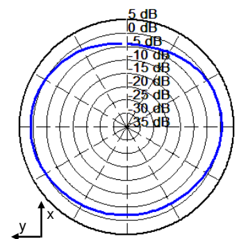
Theta = 90° Plane
