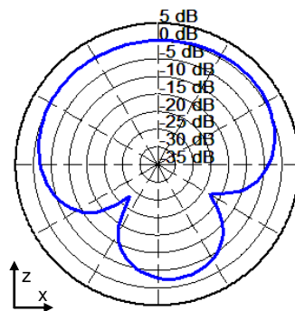
Phi = 0° Plane
