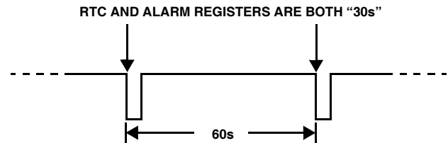
FIGURE 5. IRQ WAVEFORM
