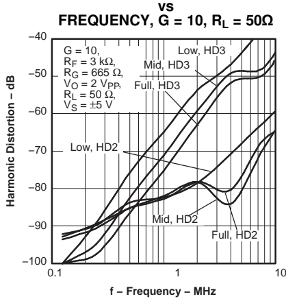
DIFFERENTIAL HARMONIC DISTORTION
