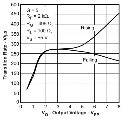
SINGLE-ENDED TRANSITION RATE
