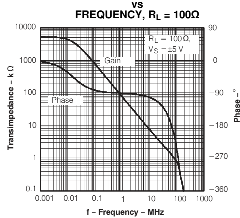
TRANSIMPEDANCE GAIN AND PHASE
