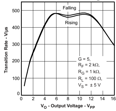
DIFFERENTIAL TRANSITION RATE
