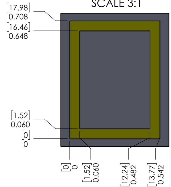
TRACE PATTERN SCALE 3:1
