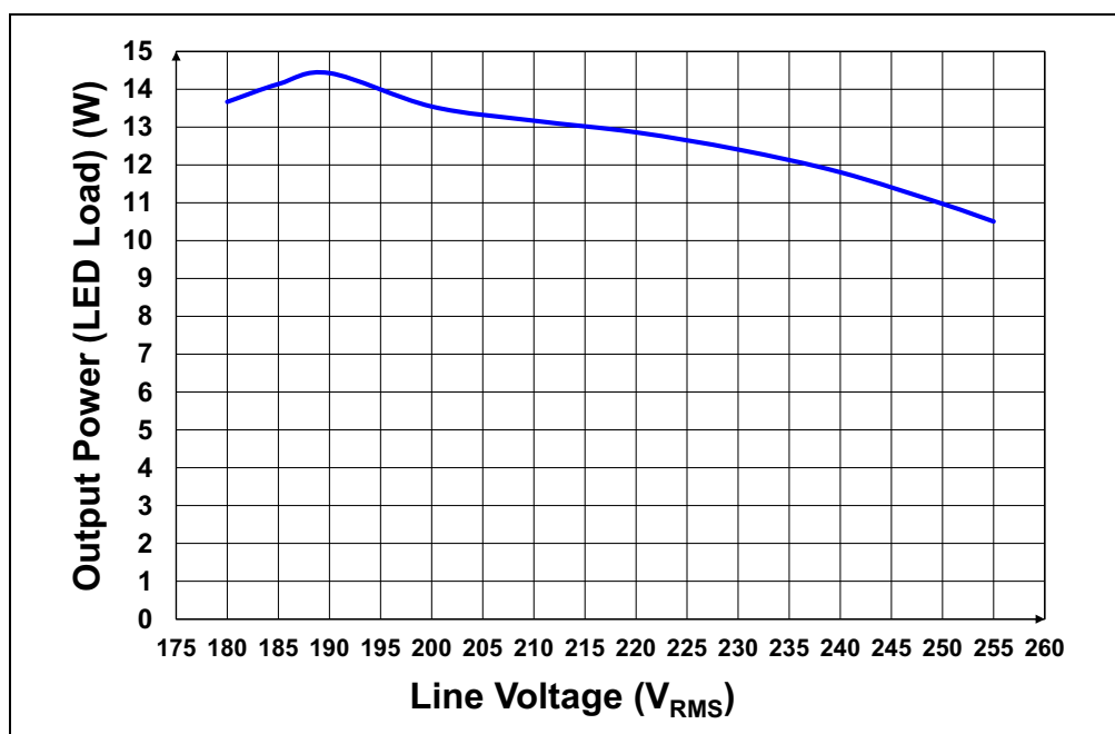
FIGURE C-15: Output Power (Electric) vs. Input Line Voltage (V RMS ).
