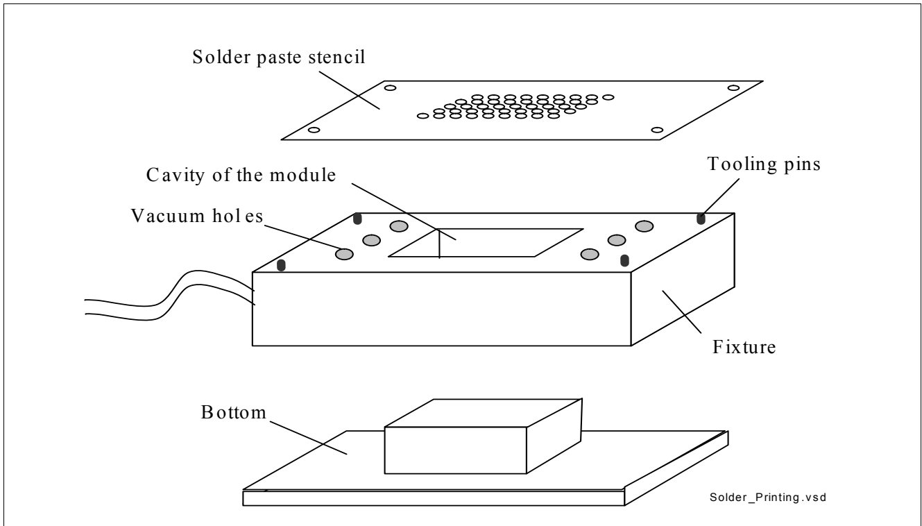
Figure 17 Solder Printing
