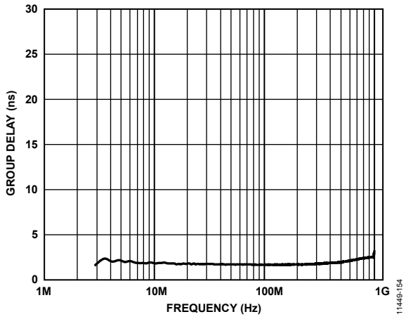
Figure 54. Group Delay vs. Frequency
