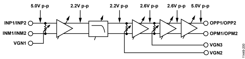
Figure 88. Maximum Signal Levels; Single Channel Shown
