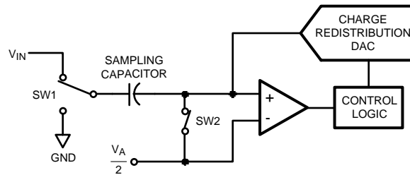
Figure 18. ADC121S051 in Track Mode
