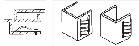
Rivet Mount
