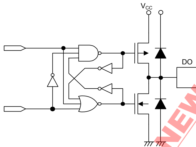
Figure 17 DO Pin
