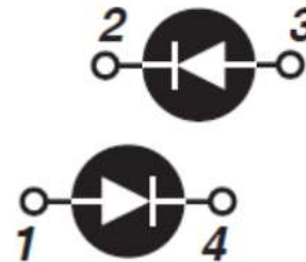
Figure 2 • Anti-parallel MSC2X100SDA070J
