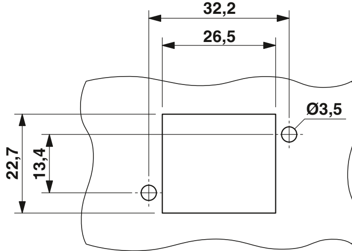
Dimensional drawing
