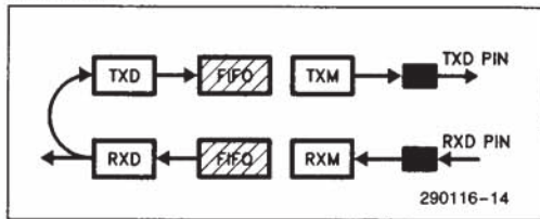
Figure 15. Auto Echo
