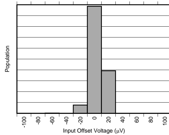
Figure 2. Input Offset Voltage Distribution (INA301A2)
