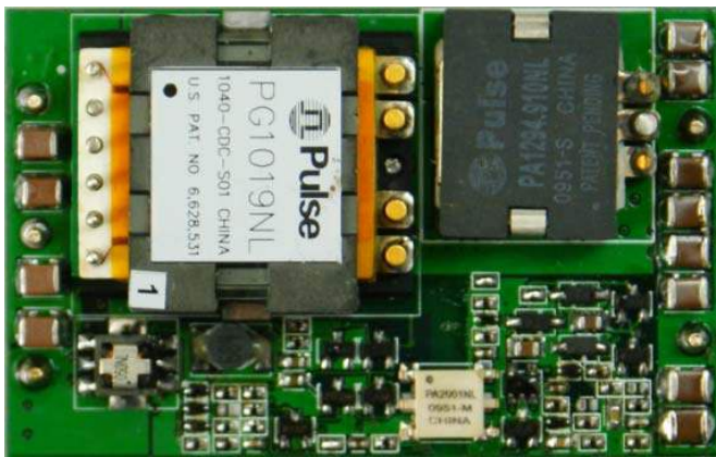
FIGURE 1. TOP VIEW OF ISL6726EVAL1Z (ACTUAL SIZE: 40x60x16mm)
