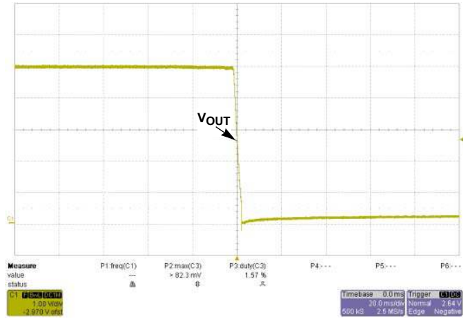
FIGURE 20. SHUT-DOWN AT V_{IN} = 36V @ I_O = 0A
