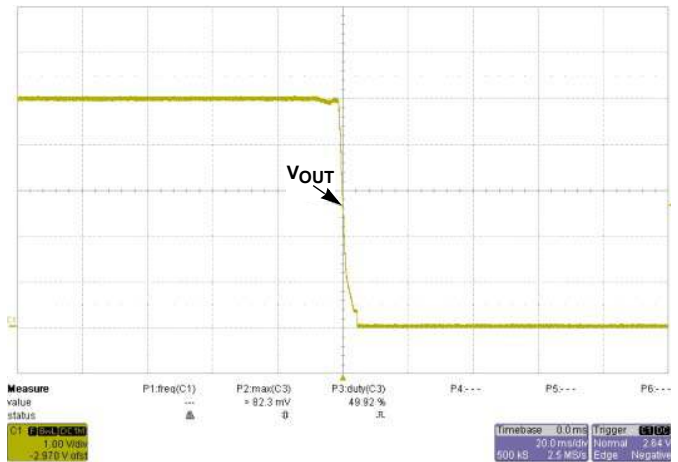
FIGURE 22. SHUT-DOWN AT V_{IN} = 36V @ I_O = 40A
