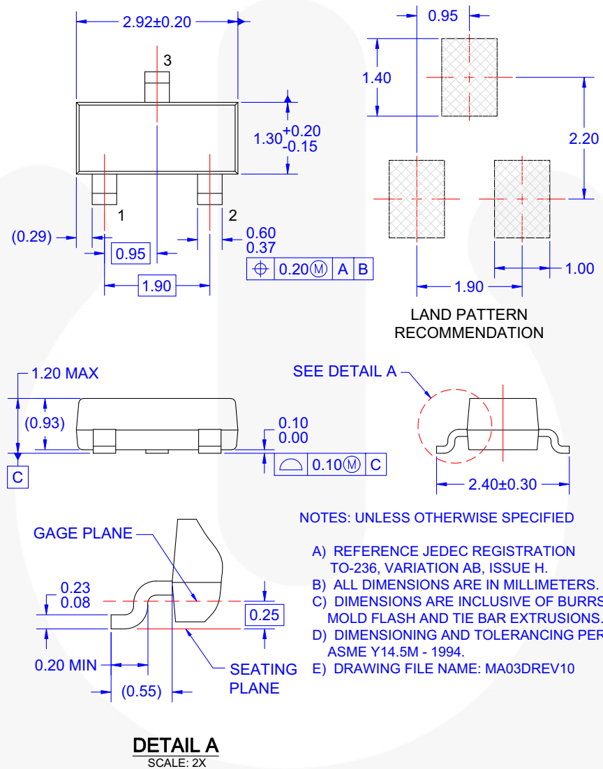
Figure 14. 3-LEAD, SOT23, JEDEC TO-236, LOW PROFILE (ACTIVE)
