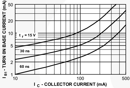
Figure 9. Rise Time vs. Turn-On Base Current
