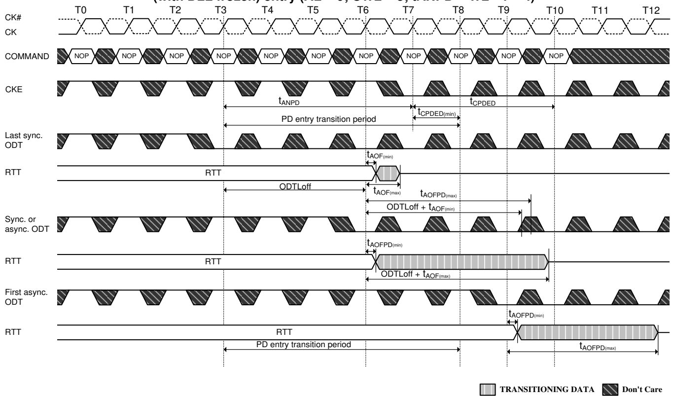
Figure 76. Synchronous to Asynchronous transition during Precharge Power Down (with DLL frozen) entry (AL = 0; CWL = 5; tANPD = WL - 1 = 4)
