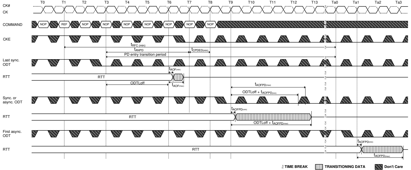
Figure 77. Synchronous to Asynchronous transition after Refresh Command (AL = 0; CWL = 5; tANPD = WL - 1 = 4)
