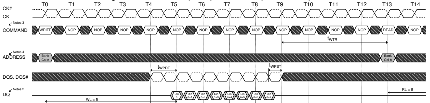
Figure 51. WRITE (BC8) to READ (BC4, BC8) OTF
