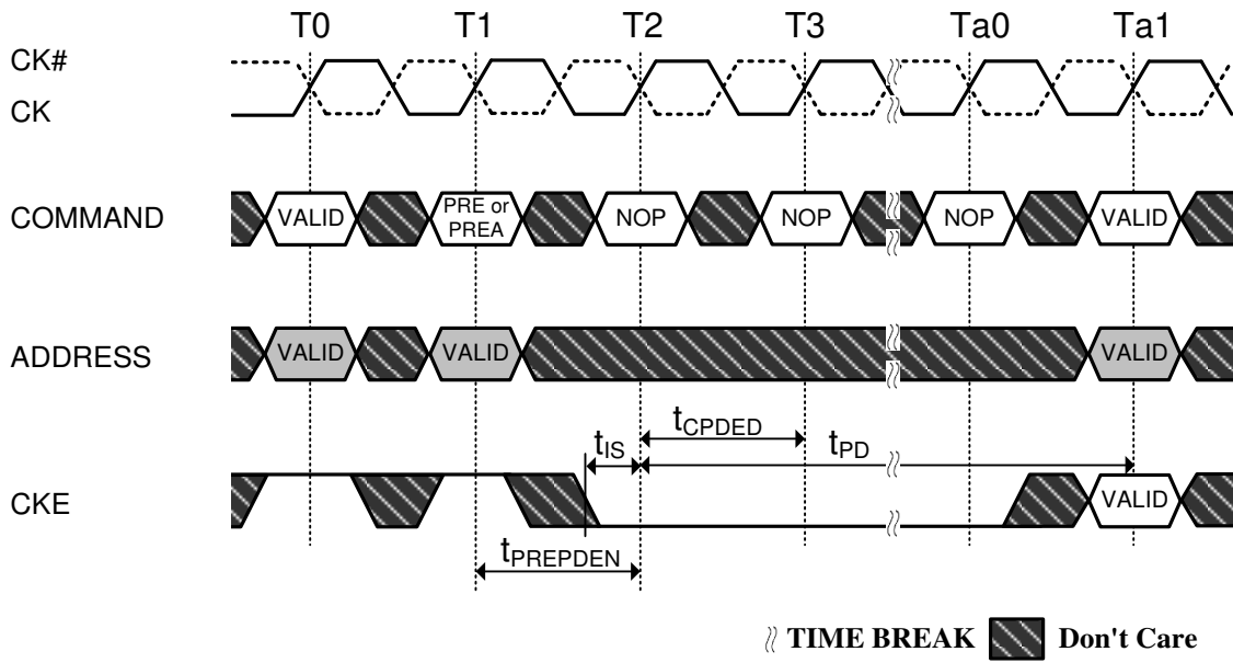
Figure 66. Precharge, Precharge All Command to Power-Down Entry
