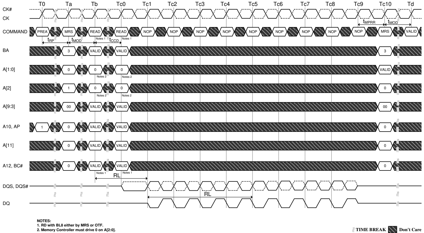
Figure 29. MPR Readout of predefined pattern, BL8 fixed burst order, back to back radout
