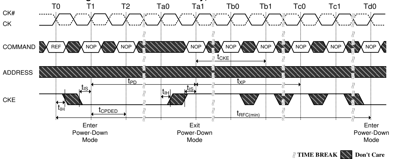
Figure 82. Power-Down Entry, Exit Clarifications-Case 3
