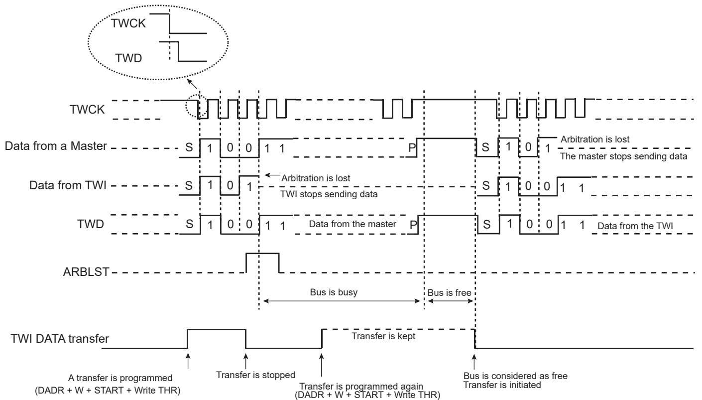
Figure 37-20: Arbitration Cases
