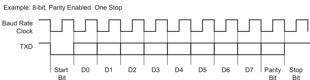
Figure 38-5: Character Transmit
