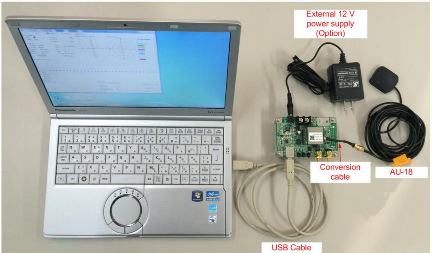
Figure 4.1 Overview of General Connection Diagram of GF-880x Series Evaluation Platform
