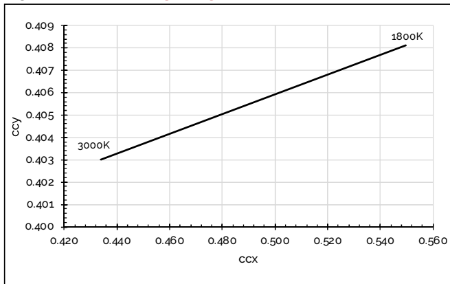
Figure 14: CCT Tuning Range, Tc=85C
