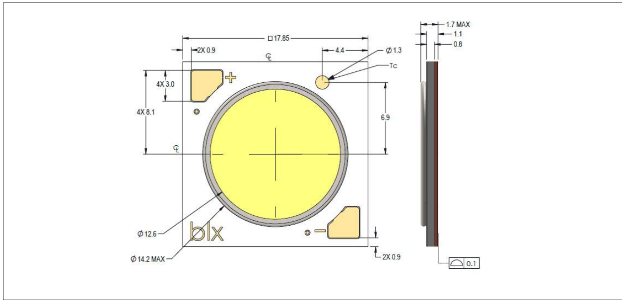
Figure 10: Drawing for H12 LED Array
