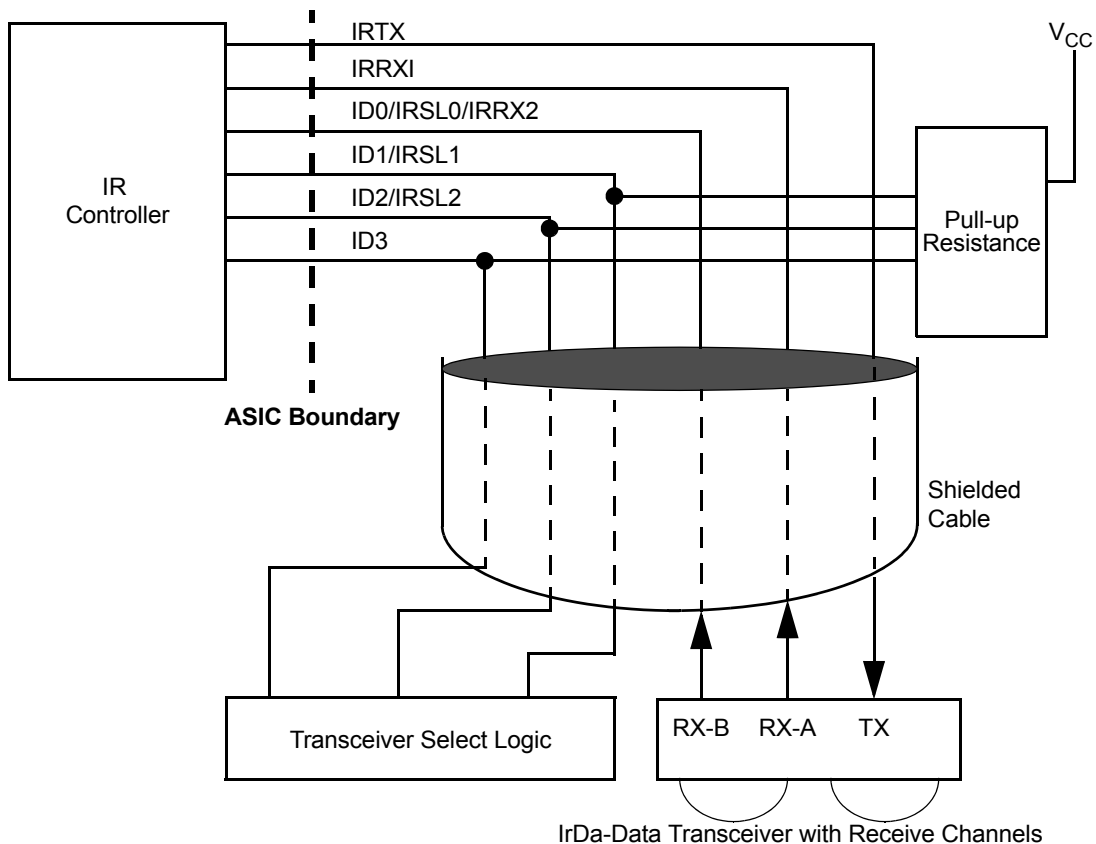
Figure 5-36. Real Dongle Interface
