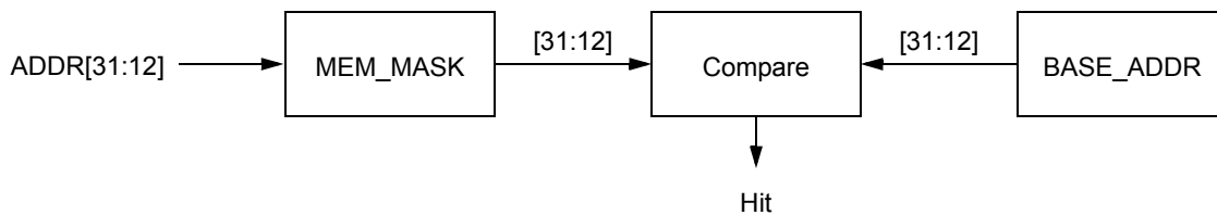
Figure 5-13. Memory Space LBAR
