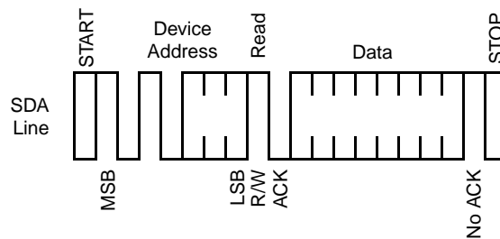
Figure 5-31. SMB Current Address Read
