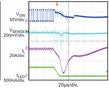
Short-Diode Protection
