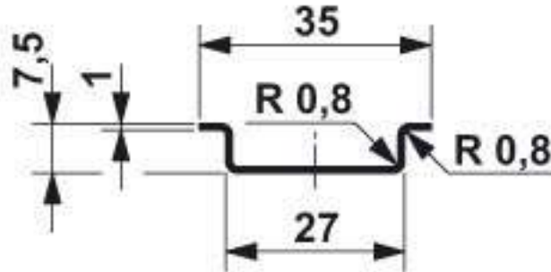
Dimensioned drawing
