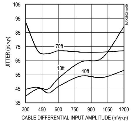
EQUALIZER RESIDUAL JITTER vs. CABLE INPUT AMPLITUDE (TENSOLITE TWIN-AX-DIFFERENTIAL)
