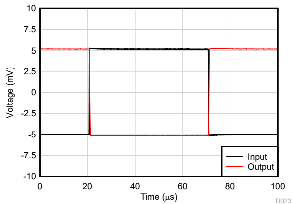
G = -1 , R_L = \text{open} , R_{FB} = 10\text{ K} See Figure 7-3
